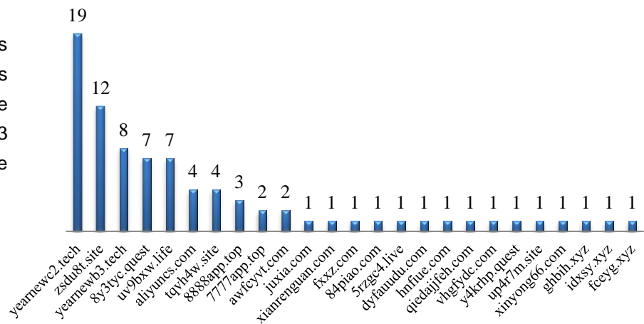
CNCERT Coordinated Platforms to Handle Mobile Malware (2/14-2/20) CNCERT/CC
